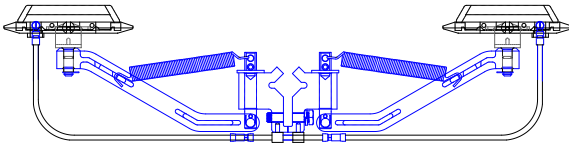
80 Amp Tandem V-Bar Collector Assembly V-80STC
