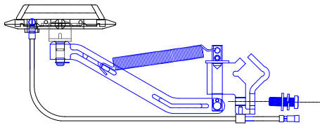
40 Amp V-Bar Collector Assembly V-40SC
